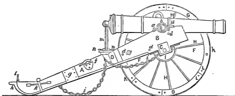
Field Gun and its Carriage:
